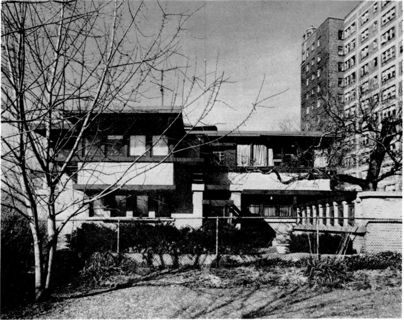
This photograph of the Bach house was taken from the neighboring lot on the south and shows the main entrance to the house (center of photograph). Unlike most residential architects of the time whose designs included a welcoming frontal entranceway, Wright chose to locate the entrance on the side of the building where it is virtually hidden from Sheridan Road. A paved walkway leads from the street, up several short flights of steps, to the rear of the property where the pavement becomes a patio. The front door, which faces the rear of the property, is entered from this patio. The location of the doorway, so unapparent from Sheridan Road, is in keeping with Wright's concern for the privacy of inhabitants of urban residences. Similarly conceived, the small casement windows are somewhat concealed beneath broad overhangs. (Barbara Crane, photographer)
